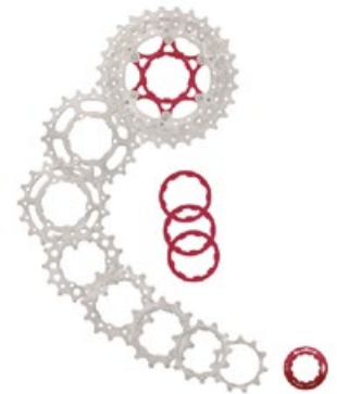
[10-Speed] [Alloy Spider] [Alloy Spacer] [Alloy Lockring] O[Black Chrome] / X[Metallic Silver] 236g[AQ] / 245g[AS] 304g[AU] / 320g[AV] / 290g [BS]
